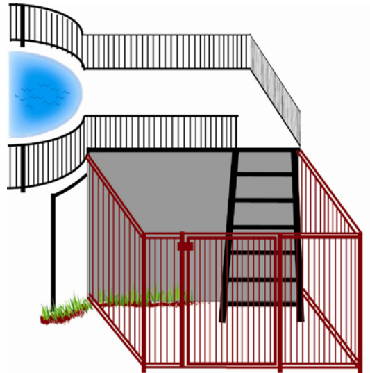
Figure 8: Above-ground pool with fenced ladder area
